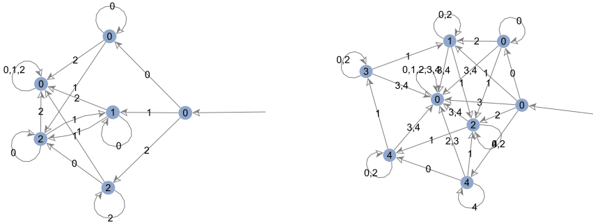
FIGURE 3.3. Automata that compute Catalan numbers modulo 3 (left) and 5 (right).
