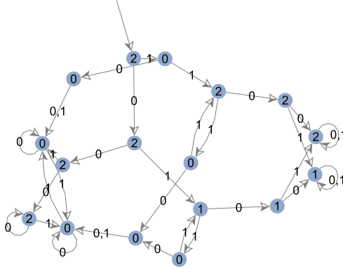
FIGURE 3.5. An automaton that computes 2-adic valuations of Motzkin numbers.
