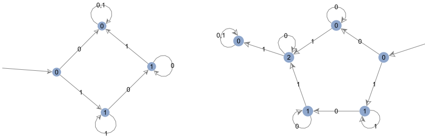
FIGURE 3.1. Automata that compute Catalan numbers modulo 2 (left) and 4 (right).
