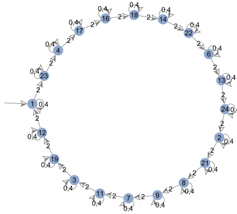
FIGURE 3.7. A subautomaton computing certain Apéry numbers modulo 25.
