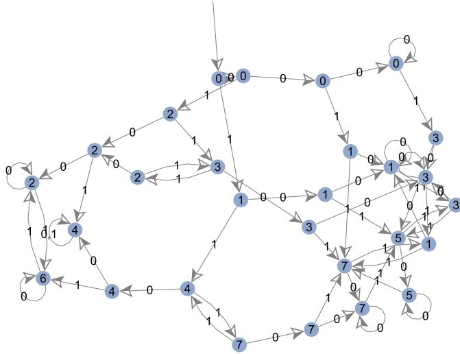
FIGURE 3.4. An automaton that computes Motzkin numbers modulo 8.
