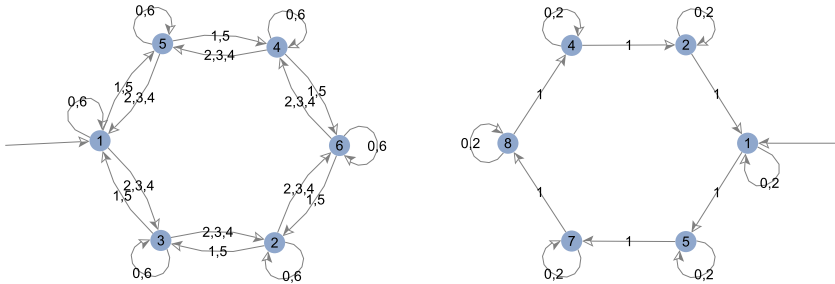
FIGURE 3.6. Automata that compute Apéry numbers modulo 7 (left) and 9 (right).
