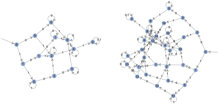
FIGURE 3.2. Automata that compute Catalan numbers modulo 8 (left) and 16 (right).
